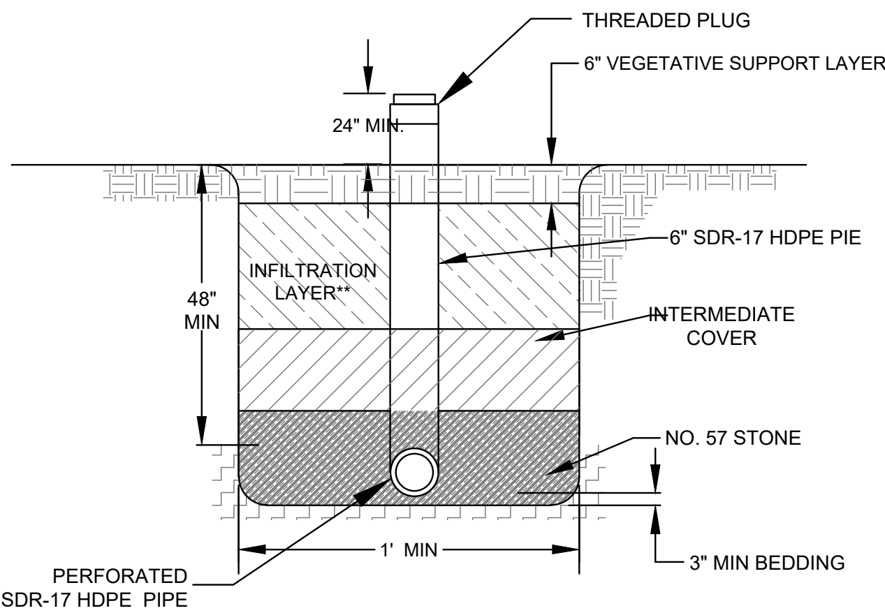
F 06 FRENCH DRAIN CLEANOUT DETAIL (TYPICAL) N.T.S.
