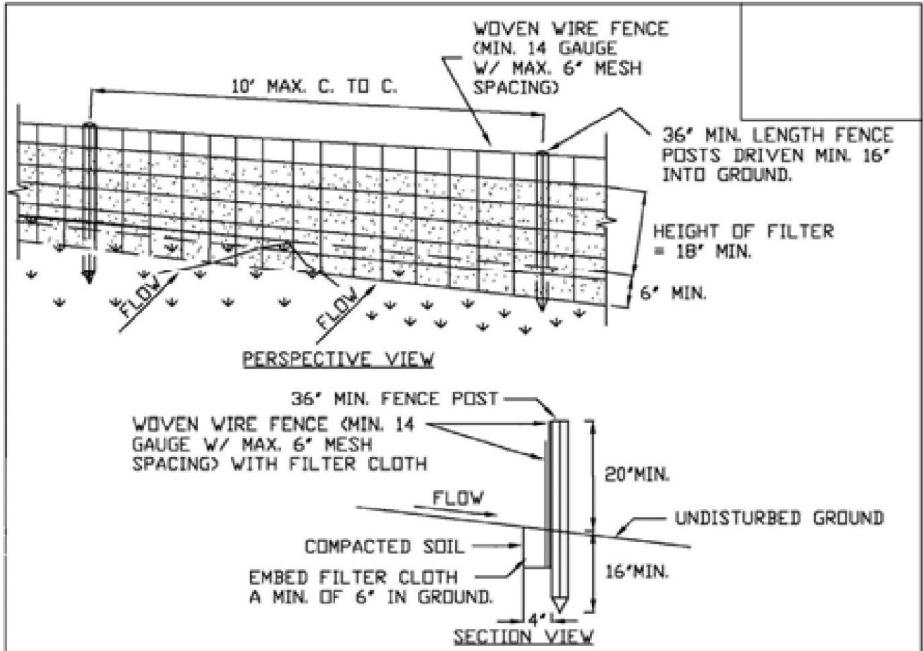
Figure 5.30 Reinforced Silt Fence
