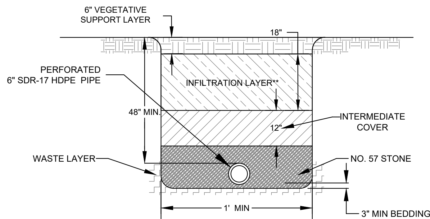
E 06 FRENCH DRAIN DETAIL (TYPICAL) N.T.S.
