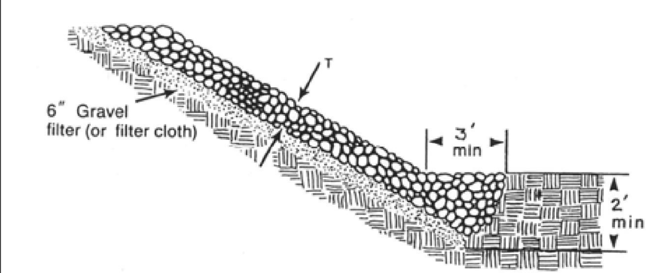
Figure 4.2 Typical Riprap Slope Protection Detail
