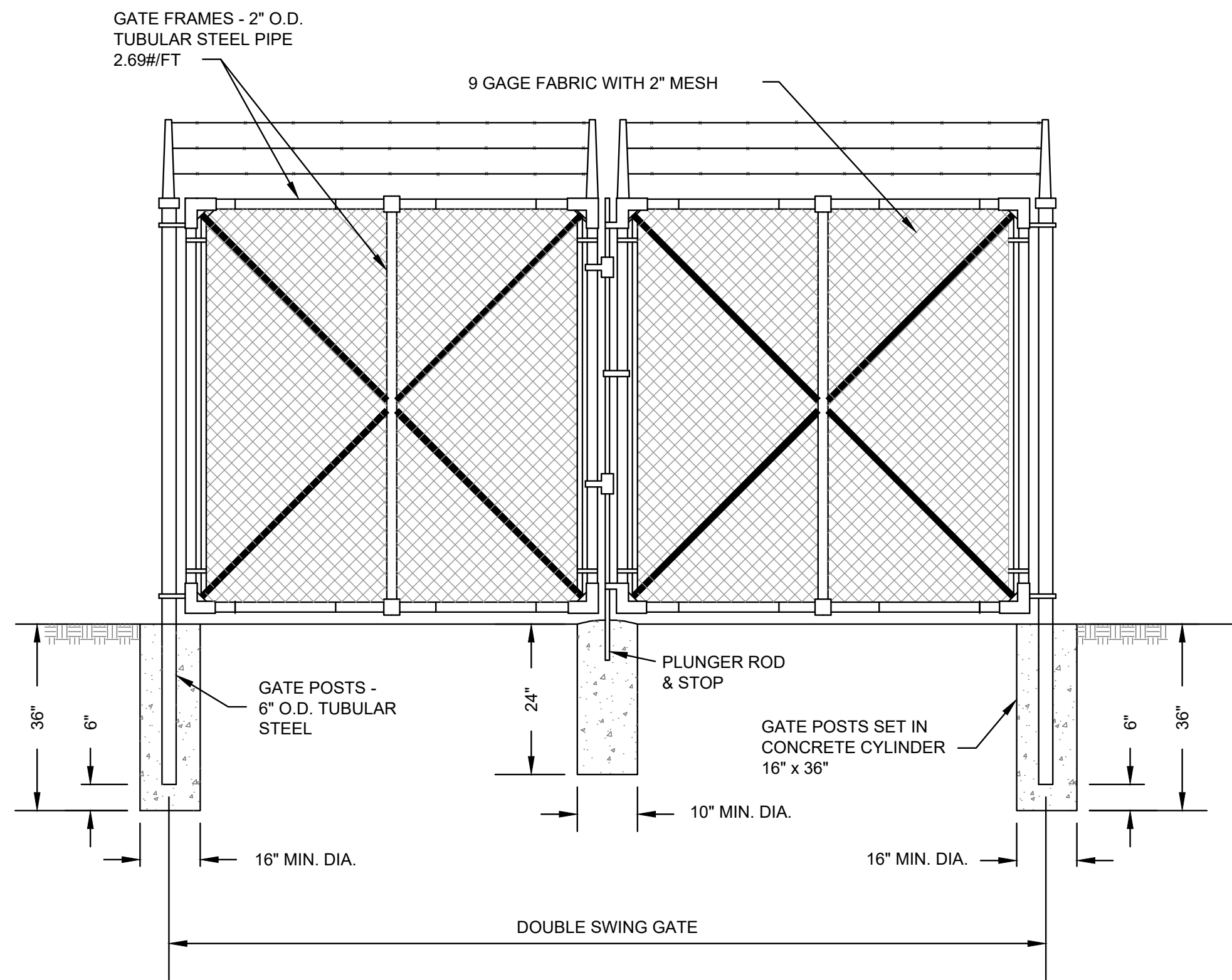
CHAIN-LINK FENCE DOUBLE GATE (I) N.T.S.
