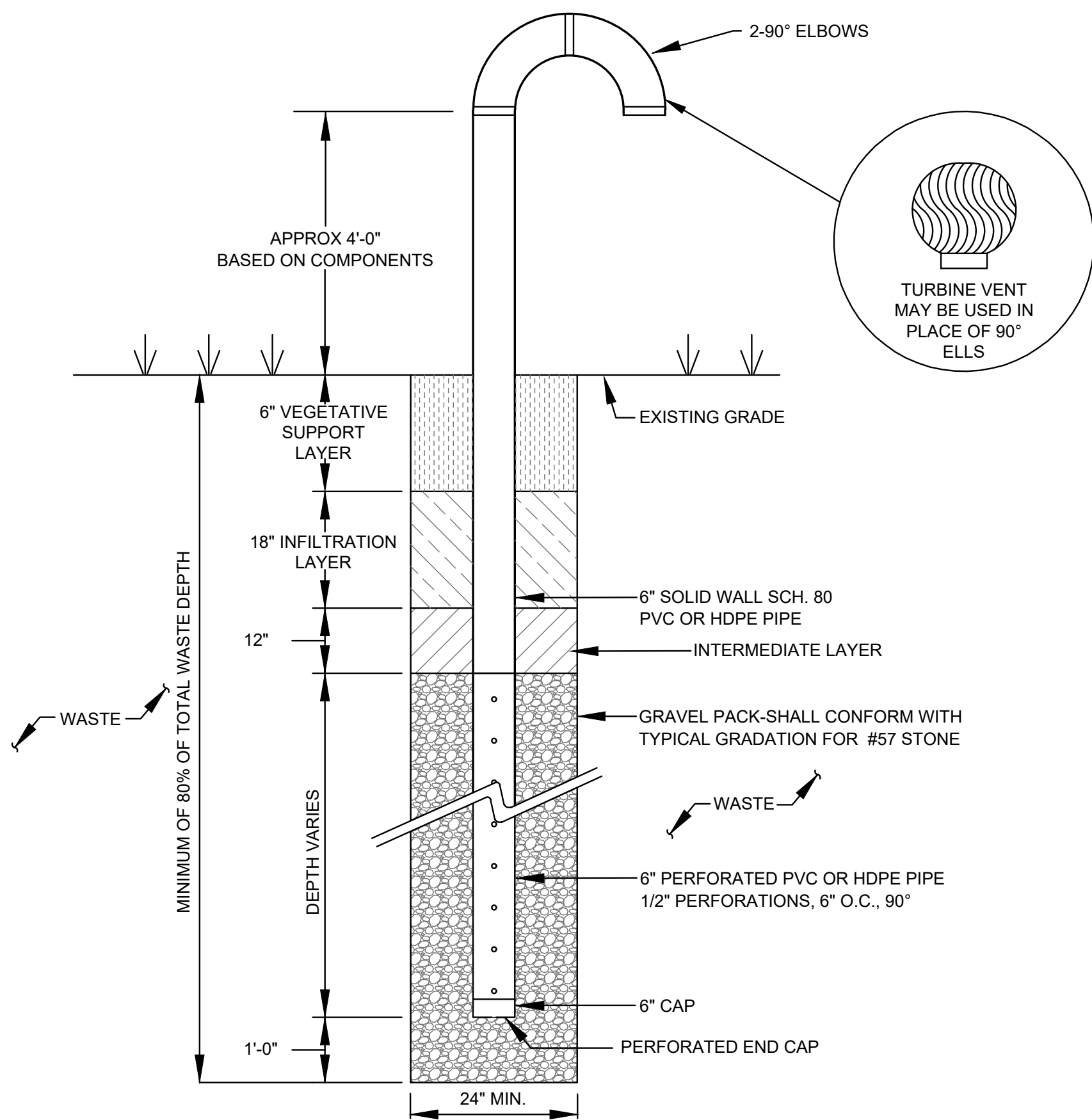
LFG PASSIVE VENT IN WASTE (J) N.T.S.
