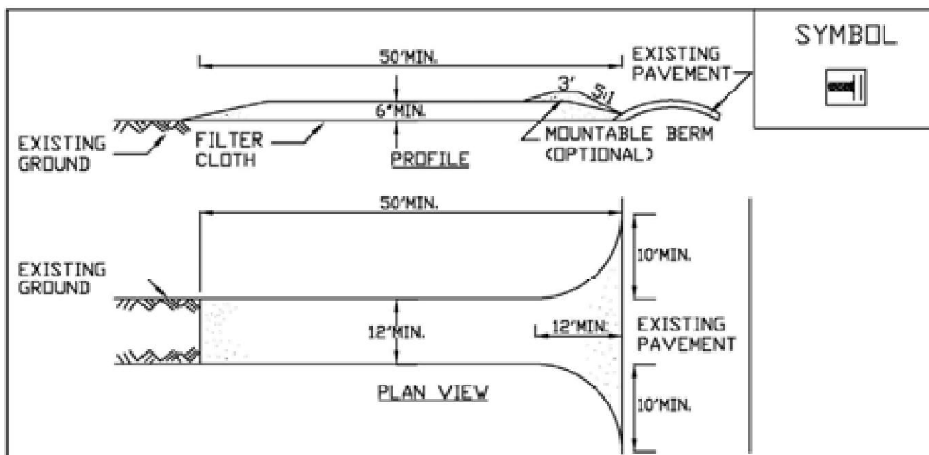
Figure 2.1 Stabilized Construction Access
